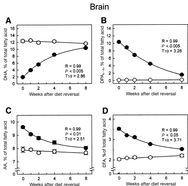
Fig. 3. Alteration in long chain polyunsaturate composition in brain after reversal of dietary n-3 deficiency. See footnotes to Fig. 1.
